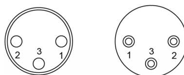
3 Pin XLR
