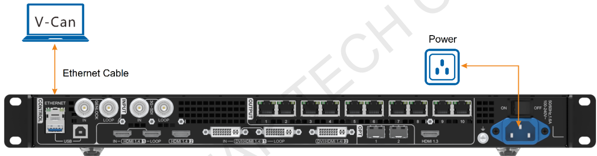
Figure 6-1 Hardware connection
